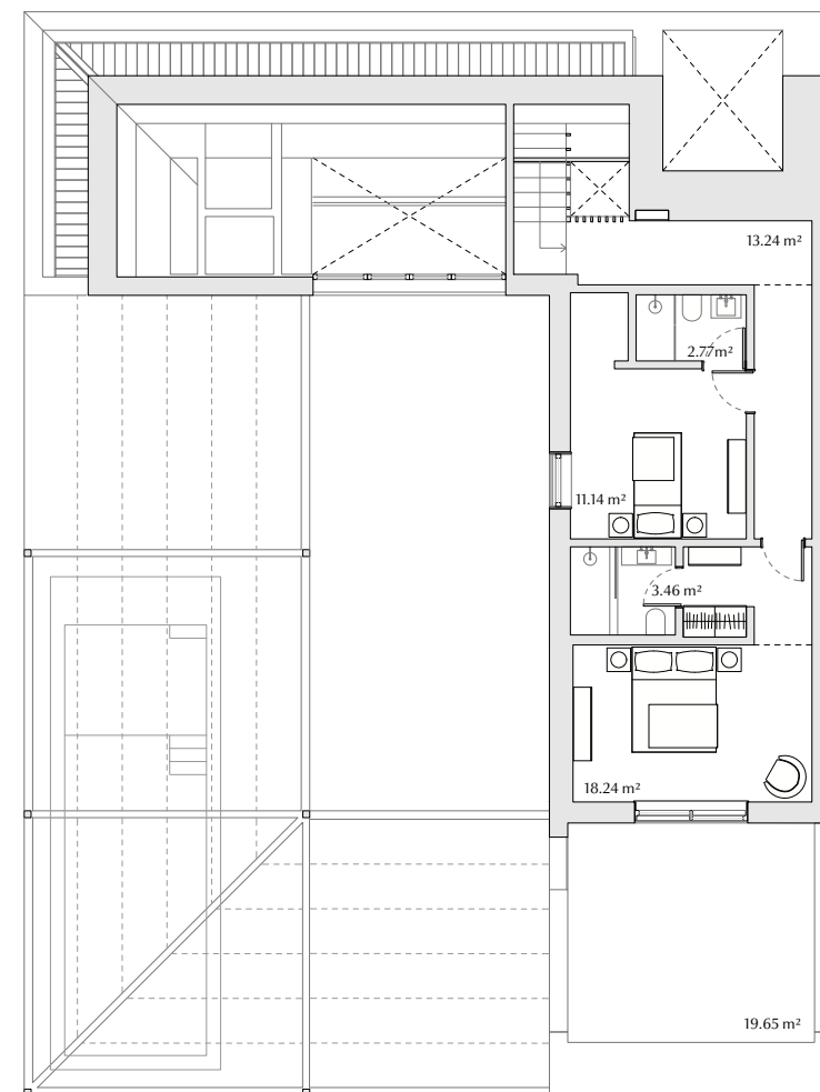
SECOND FLOOR
