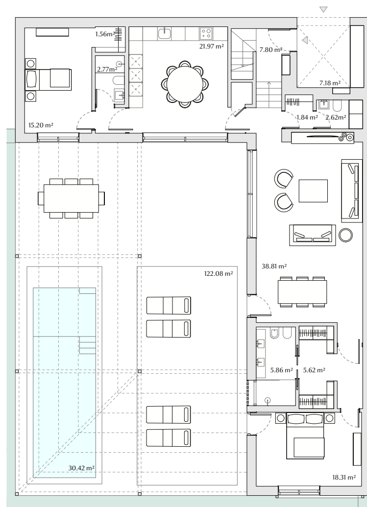
FIRST FLOOR
